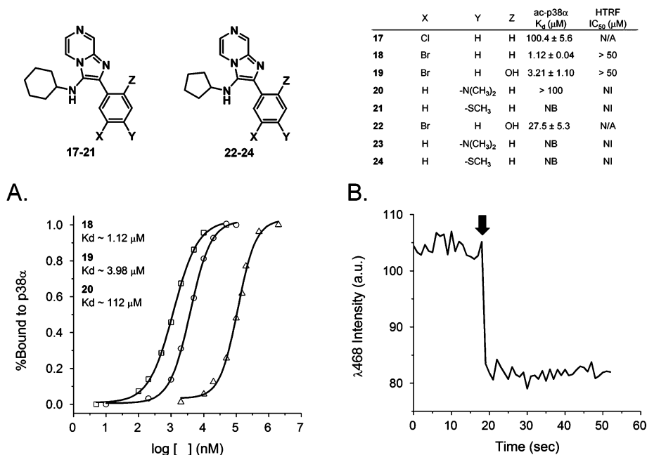
Figure 4. SAR and characterization of 17 , 22 , and close derivatives using acrylodan-labeled p38 \alpha . Two hits from the HTS screen, 17 and 22 , were not commercially available (N/A) for testing in an activity-based assay. Therefore, several close derivatives ( 18–21 , 23 , 24 ) were obtained for IC 50 determinations and for performing SAR studies on this identified scaffold (top panel). Compounds 21 , 22 , and 24 were not detected by acrylodan-labeled p38 \alpha (NB; no binding). Compounds 20 , 21 , 23 , and 24 were not detected in HTRF assay (NI; no inhibition). There was a clear preference for compounds with a meta -halogen substituted phenyl ring. As was the case with several other hit compounds, these derivatives have a much weaker effect in the activity-based assay in which the phosphorylated kinase is used. Acrylodan-labeled p38 \alpha binding assay was used to determine the K d of several compounds, including 18 ( \square ), 19 ( \circ ), and 20 ( \triangle ) (B). Real-time kinetic measurements of 18 reveal a rapid decrease ( t_{1/2} < 5 s) in the fluorescence emission of acrylodan at 468 nm, indicative of the binding of a Type I ligand (C). The detection of this compound suggests that the compound may promote the DFG-out conformation despite binding primarily within the ATP binding site as observed for other Type I p38 \alpha inhibitors. 7 All fluorescence traces and binding curves are representative of at least three independent measurements.
