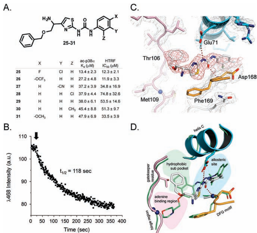
Figure 6. Characterization of the identified p38 \alpha 2,5-disubstituted thiazole-urea inhibitors 25–31 . K_d and IC 50 values determined with the acrylodan-labeled kinase binding assay and the HTRF assay, respectively, are shown along with the general chemical structure of these compounds (A). Upon addition of 25 (black arrow) to a rapidly stirred suspension of acrylodan-labeled p38 \alpha , a slow decrease ( t_{1/2} = 118 s) in acrylodan fluorescence was observed at 468 nm, indicating slow binding to the DFG-out conformation of p38 \alpha (B). All other compounds produced a similar slow binding kinetic (not shown). Cococrystallization of 25 with p38 \alpha revealed that the ligand is located completely within the allosteric pocket in a Type III binding mode (C). The phenyl moiety is buried inside the hydrophobic subpocket located beyond the gatekeeper residue. This moiety is conserved in all thiazole-urea compounds identified in the high-throughput screen suggesting it is a crucial contributor to affinity. The urea moiety forms the expected hydrogen bonding interactions with the DFG motif and the side chain of Glu71 of helix C (red dotted lines). The identification of these thiazole-urea compounds as ligands which bind within the allosteric pocket of p38 \alpha represents a novel binding mode for this class of compounds. The benzyl moiety of the inhibitor binds into the hydrophobic subpocket flanked by the gatekeeper Thr106 and forces the inhibitor to adopt a constrained conformation when compared to the binding mode of the Type II inhibitor BIRB-796 11 (green thin sticks) (D). The allosteric site, hydrophobic subpocket, and the adenine binding region are color coded. The shown fluorescence trace is representative of at least three independent measurements. All K_d and IC 50 values represent the mean \pm s.d. of at least three independent measurements.
